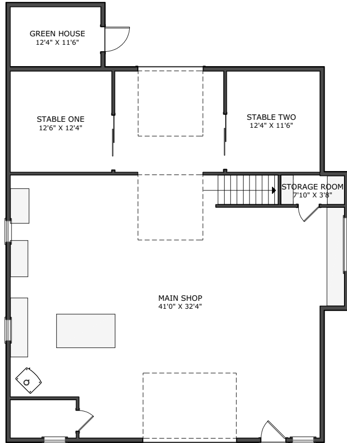
MAIN LEVEL
